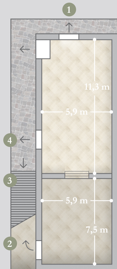
GROUND FLOOR Floor surface: 110,9 m 2
