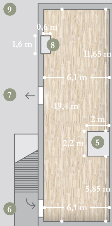
FIRST FLOOR Floor surface: 113,9 m 2
